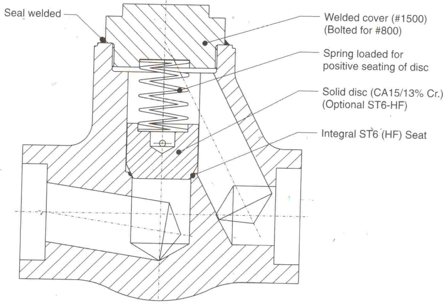
Check Valve
