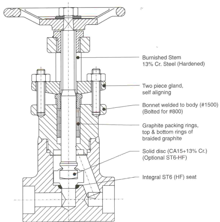
Globe Valve
