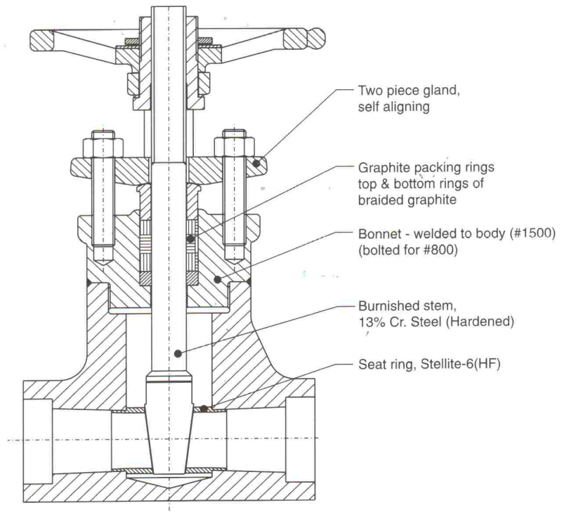
Gate Valve
